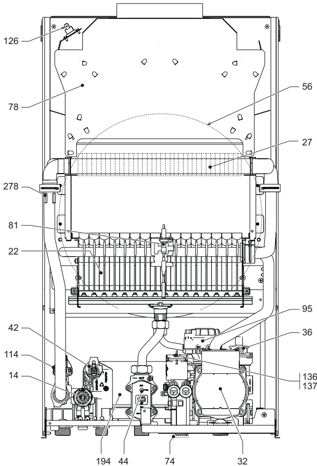
fig. 21- General view - DIVAtch D LN C30
