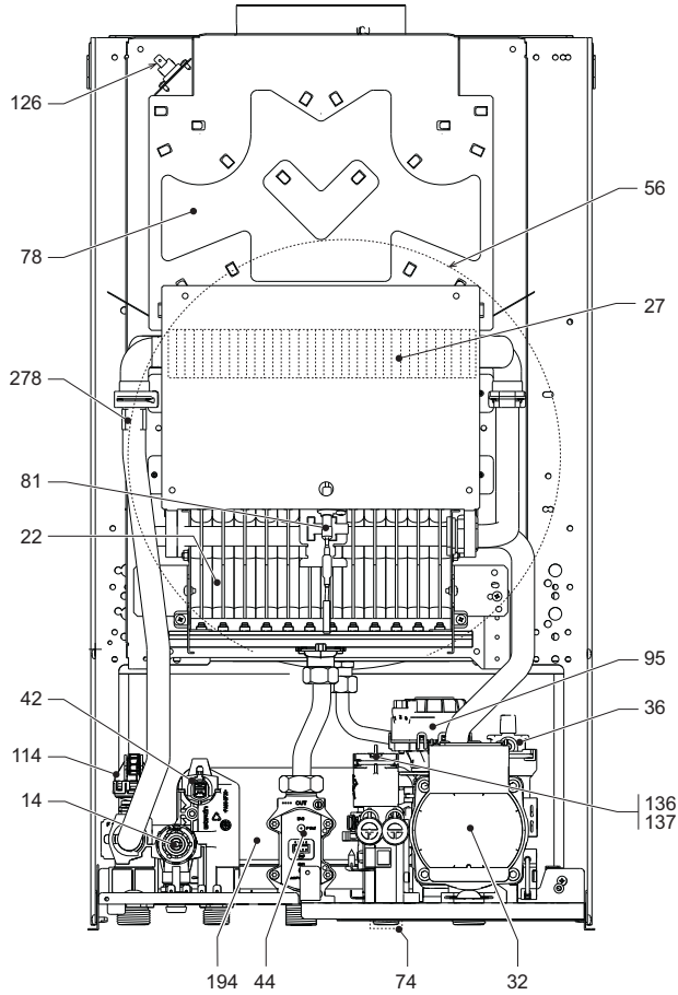
fig. 20- General view - DIVAtch D LN C24
